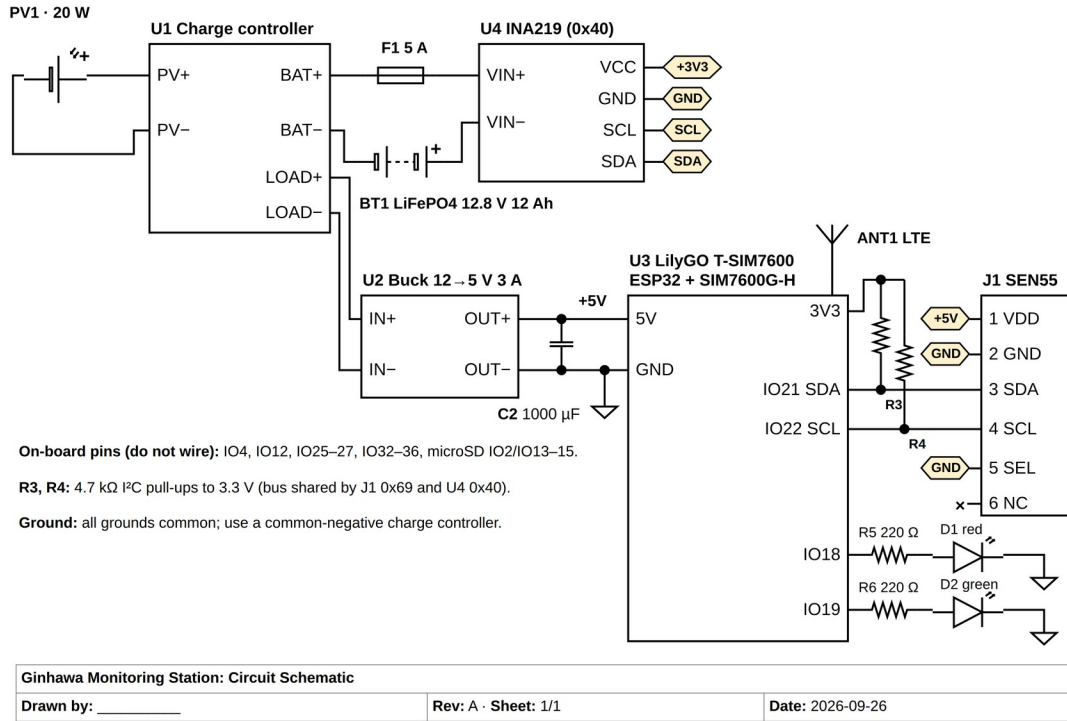
Figure 8. Circuit Diagram
