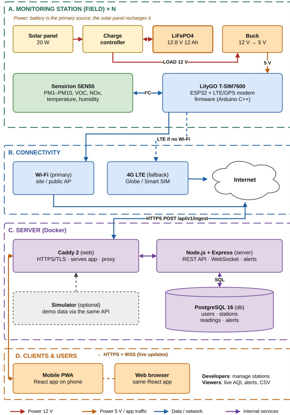
Figure 2. System Architecture Diagram
