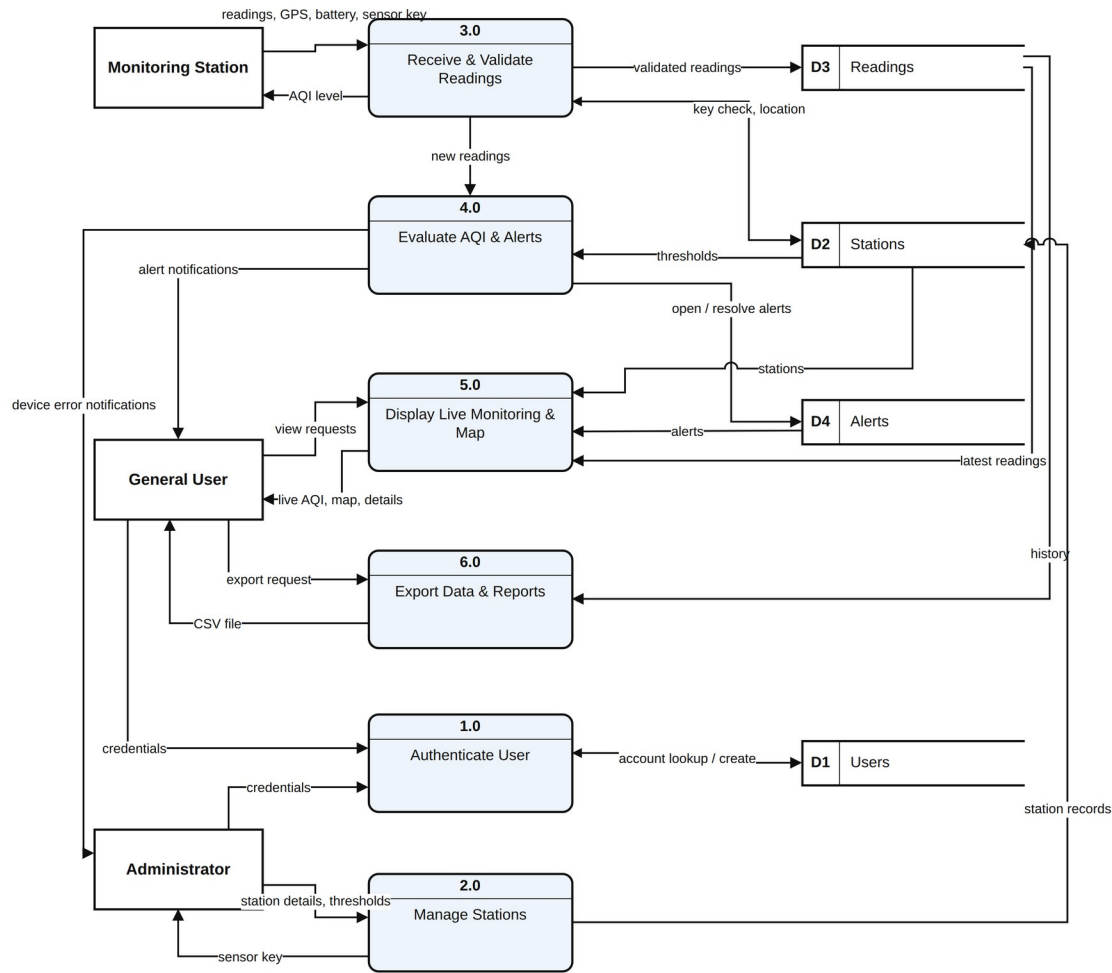
Figure 6. Level 1 Data Flow Diagram
