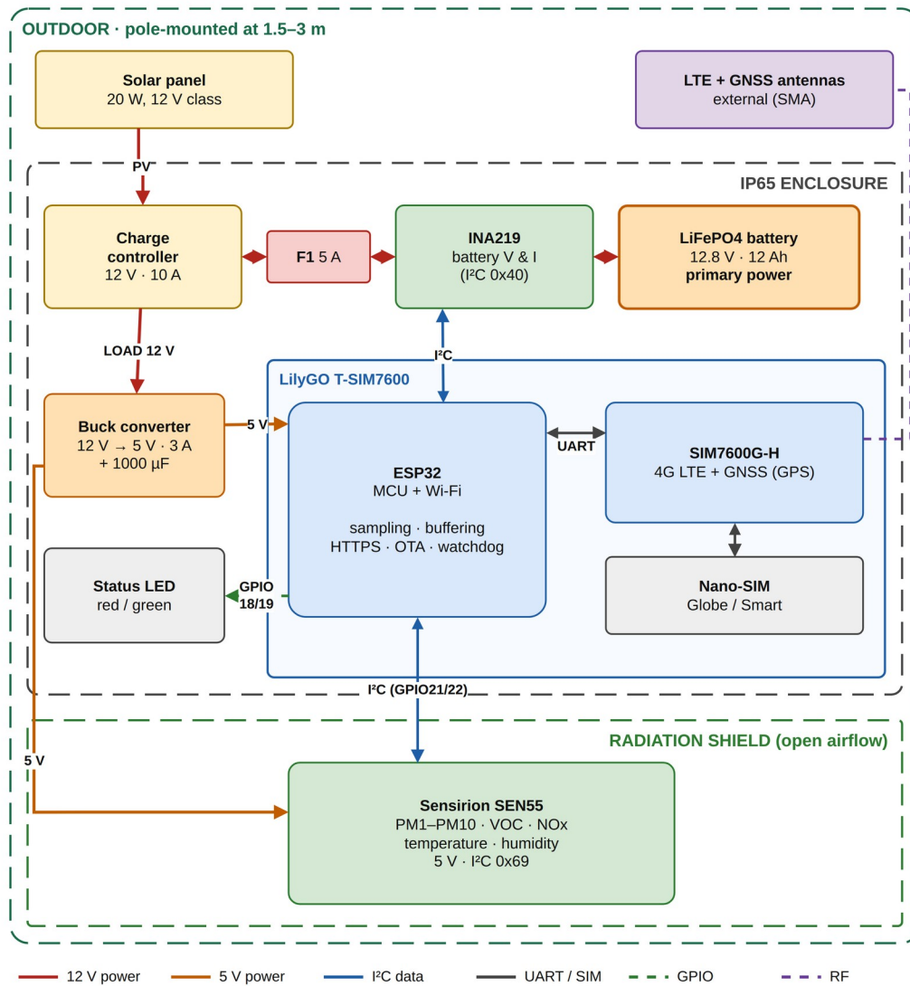
Figure 7. Monitoring Station Hardware Block Diagram
