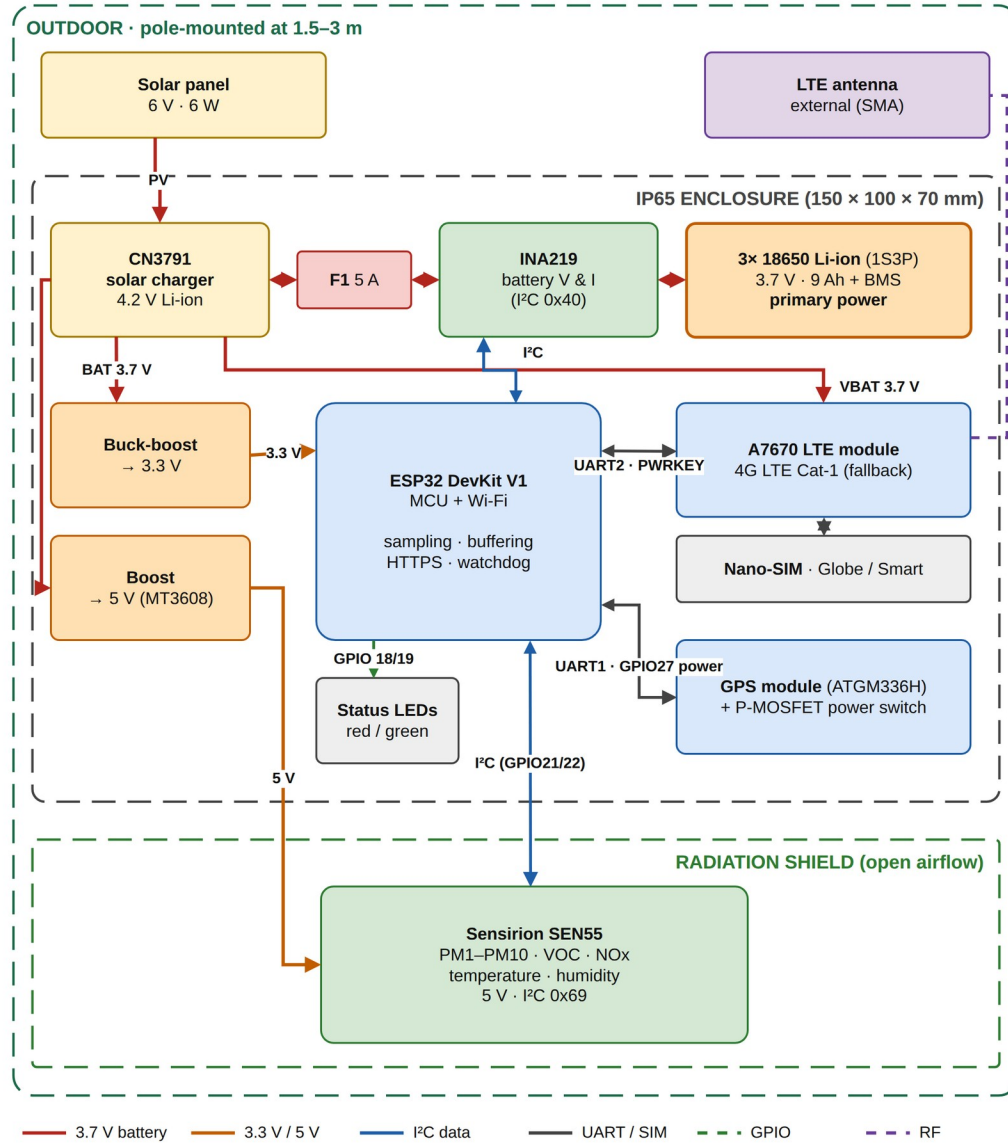
Figure 7. Monitoring Station Hardware Block Diagram
