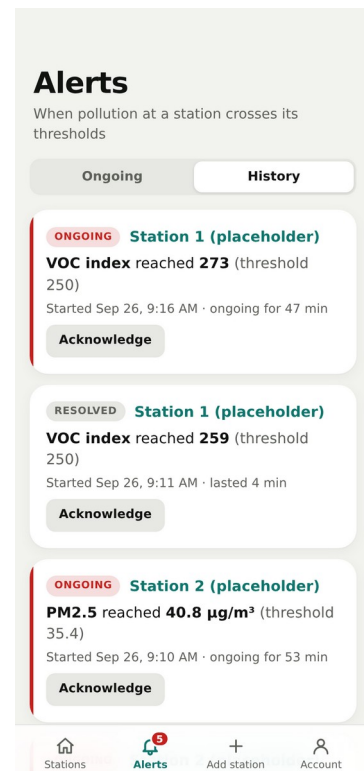
Figure 12. Alerts
