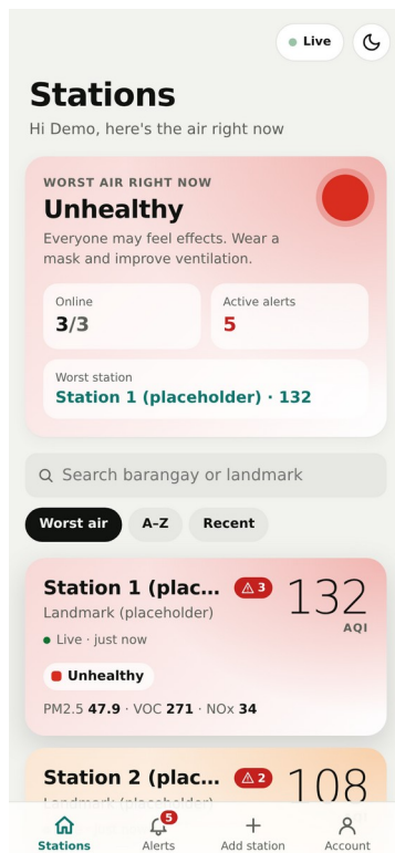
Figure 10. Stations Dashboard
