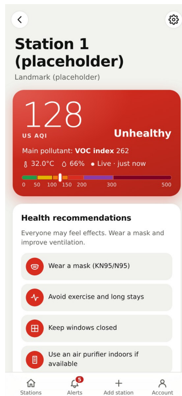
Figure 11. Station Details
