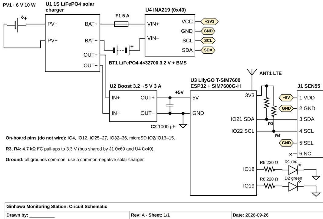
Figure 8. Circuit Diagram
