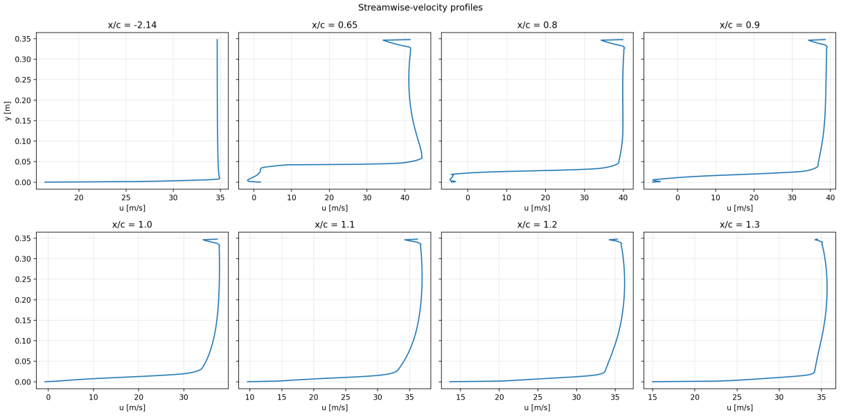
Figure 2: Third-pass velocity-profile set at the validation stations.
