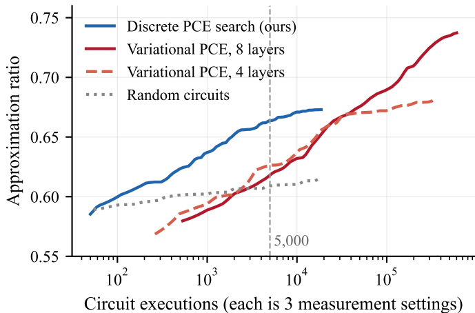
(b) 858 variables on 13 qubits, mean over instances and runs
