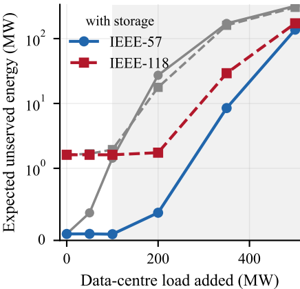
Unserved energy under N-1
