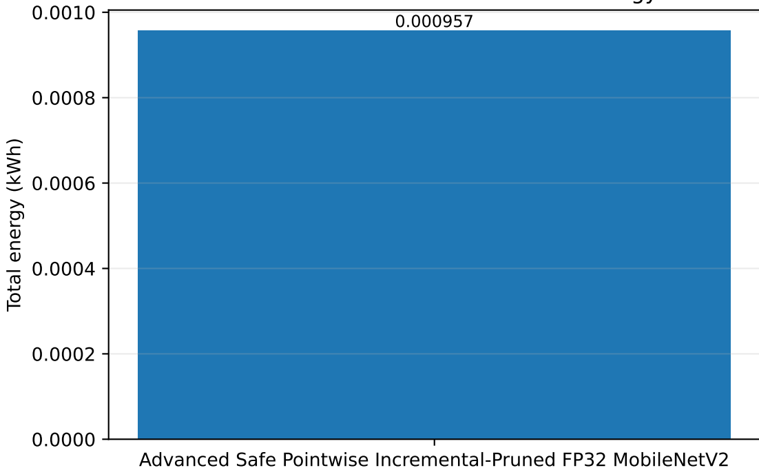
Advanced Pruned Total Inference Energy
