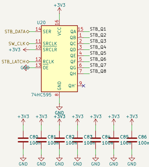
74HC595 strobe register
