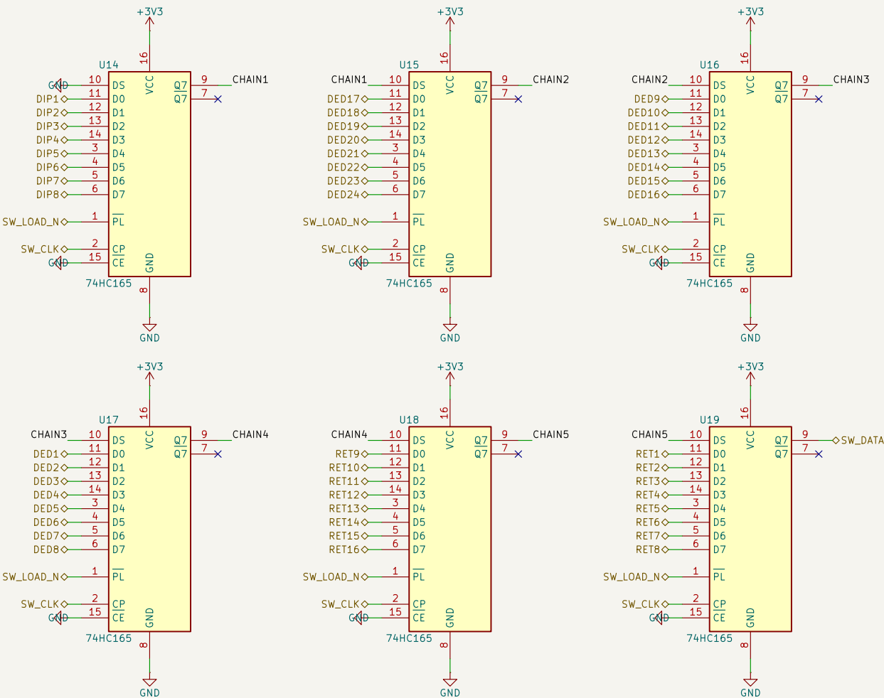
74HC165 input chain (3.3 V)
