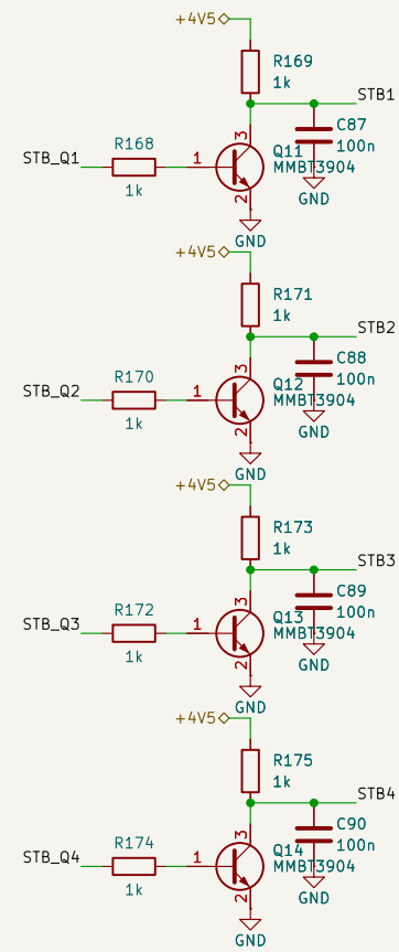
Strobe drivers 1–4
