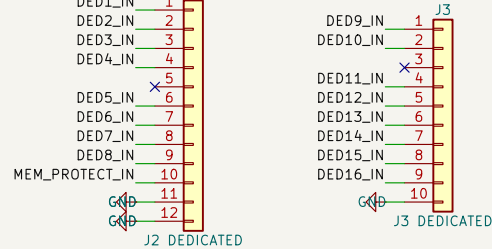
Connectors J2, J3, J13
