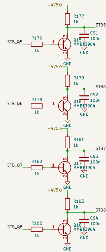
Strobe drivers 5–8
