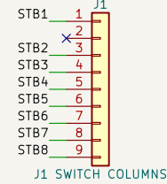
J1: switch columns (strobes)
