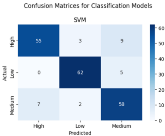
Figure 11: Confusion matrix of the SVM classification model
