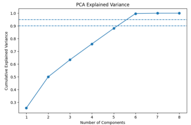
Figure 7: Principal Component Analysis
