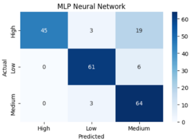
Figure 13: Confusion matrix of the MLP Neural Network
