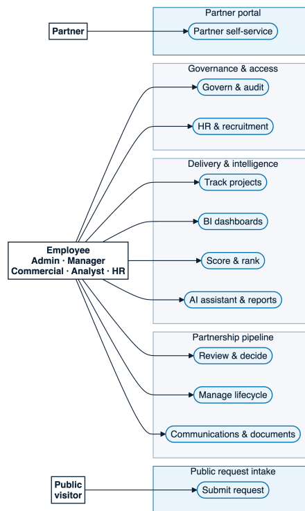
Figure 2.1: Global use-case diagram of IntelliConnect
