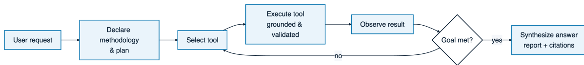
Figure 6.1: The agentic reasoning loop of the IntelliConnect assistant.
