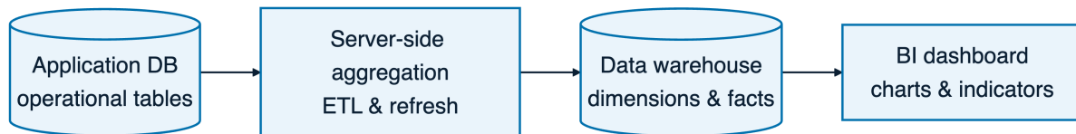
Figure 5.4: Application database to data warehouse flow.
