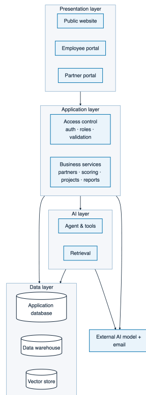
Figure 2.4: Feature-driven monolith architecture of IntelliConnect
