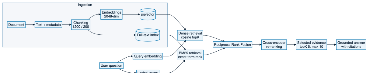
Figure 7.2: RAG ingestion and retrieval pipeline
