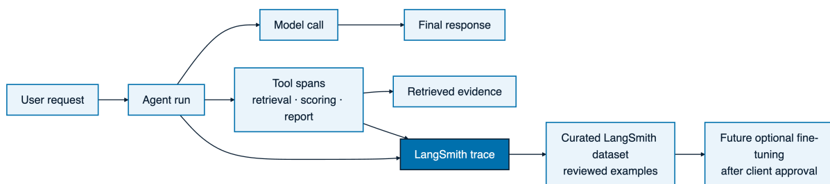
Figure 7.5: Observability trace flow of an agent run
