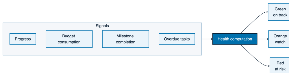
Figure 5.3: Project health computed from delivery signals.
