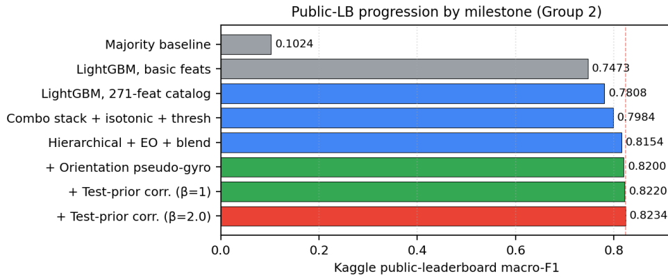
Fig. 3. Public-LB macro-F1 by milestone (Group 2). Feature engineering and calibration drive the rise to 0.8154; the data-physics ideas (orientation pseudo-gyroscope, test-prior correction) add the final +0.008 to reach 0.8234.
