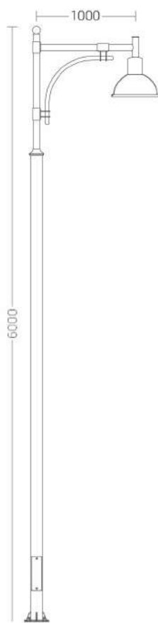
Emperor Pole LXP-2208
