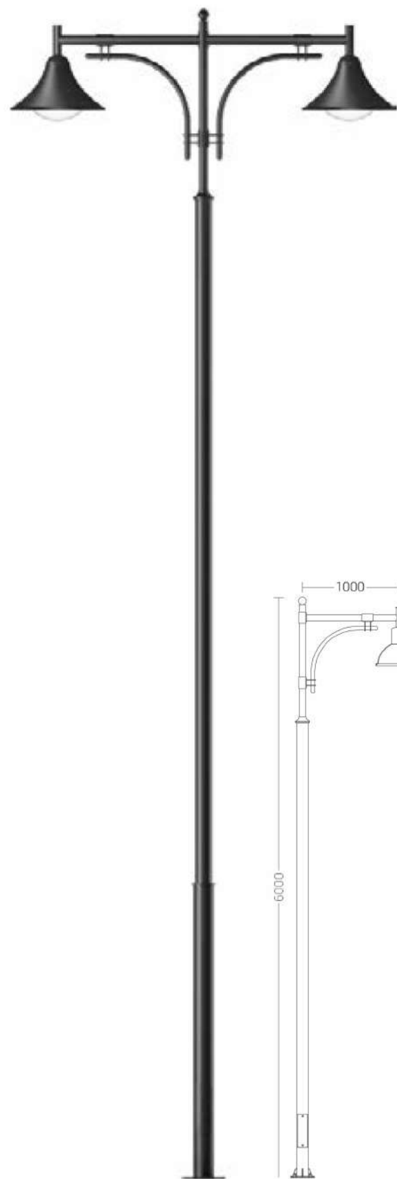
Emperor Pole LXP-2208
