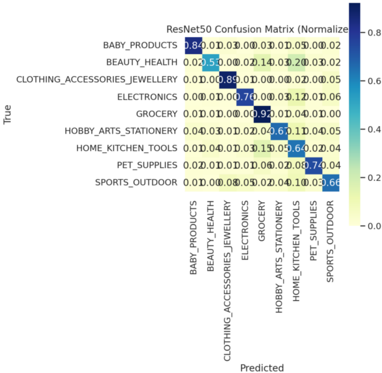
Figure 4 Confusion Matrix Resnet50 Normalized
