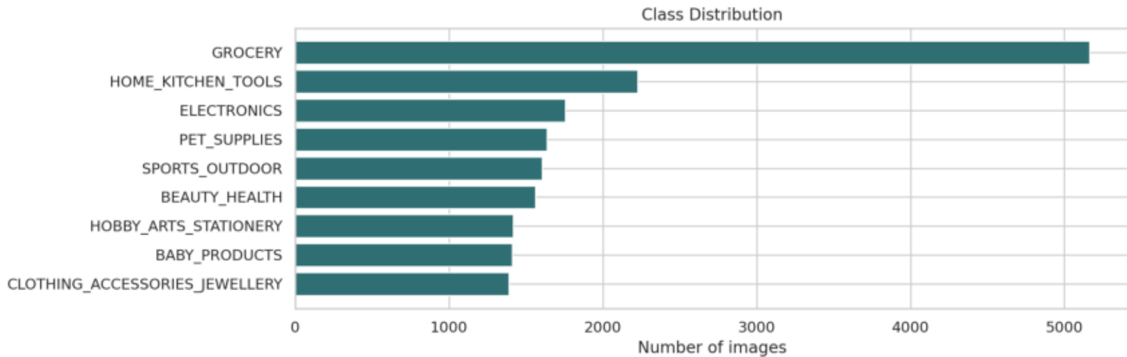
Figure 1A Class Distribution
