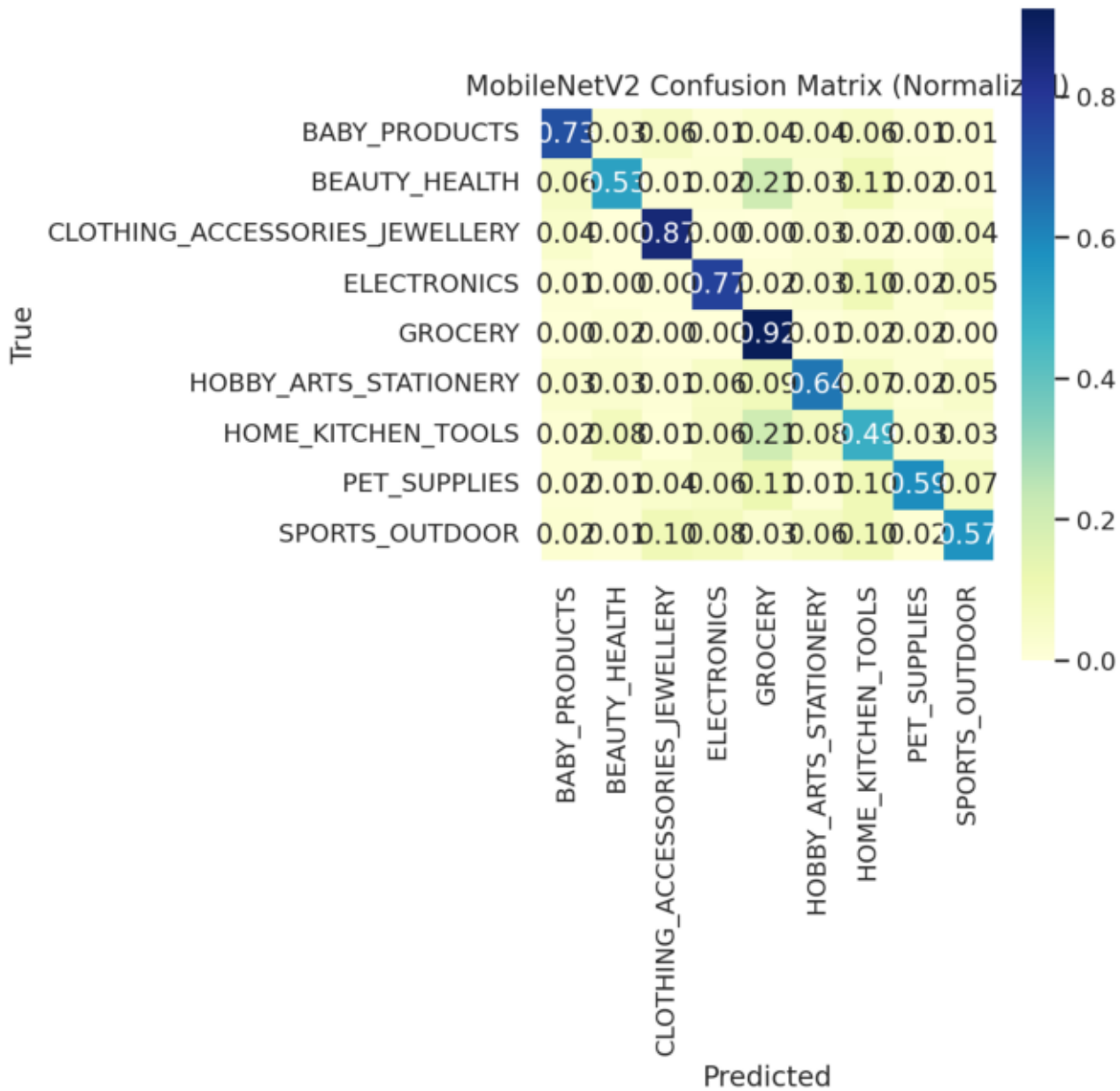
Figure 4 Confusion Matrix Mobilenetv2 Normalized
