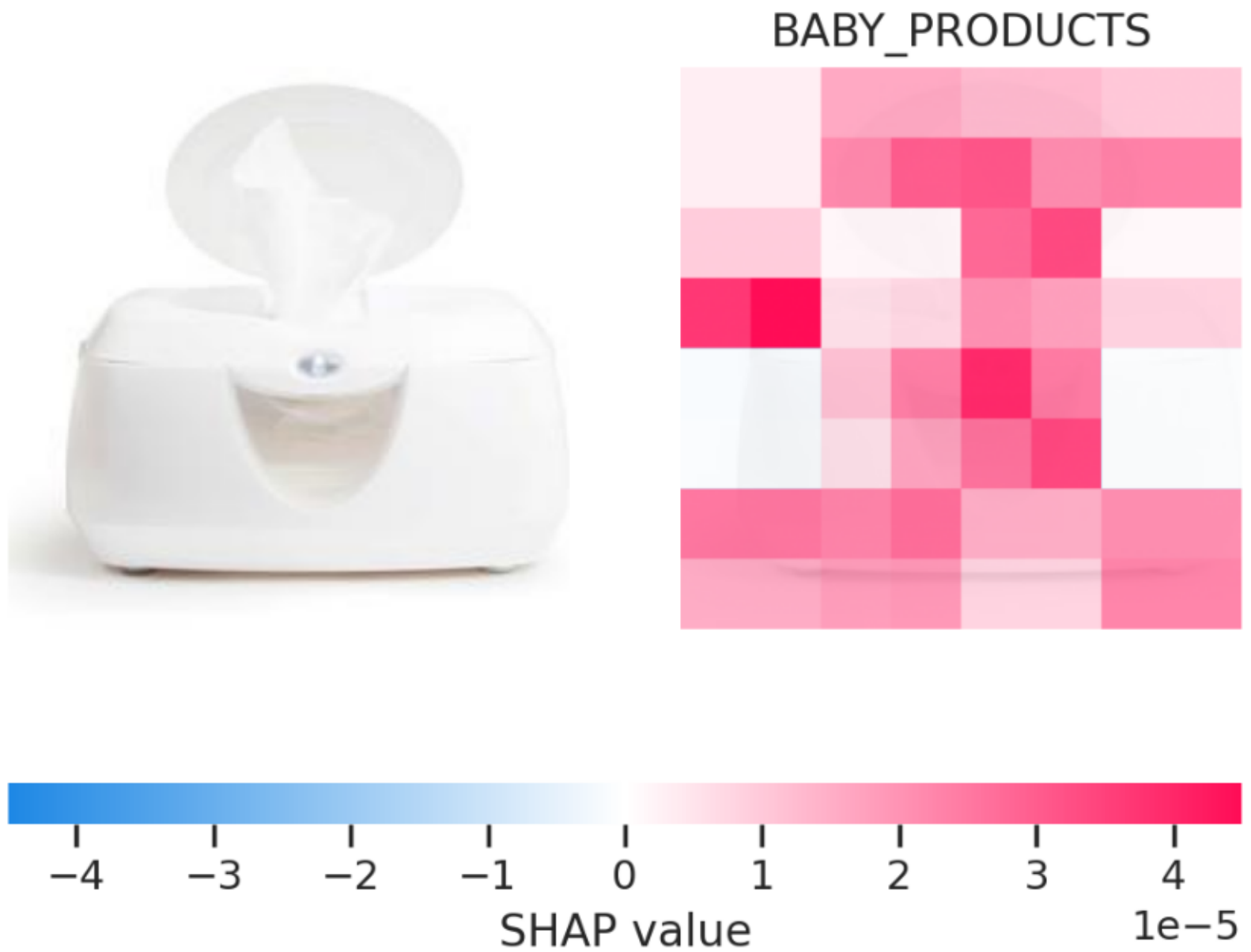
Figure 7 Shap Mobilenetv2
