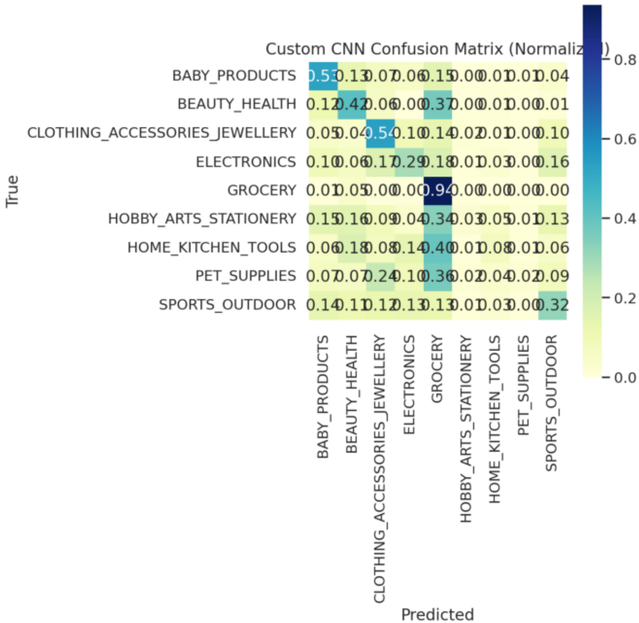
Figure 4 Confusion Matrix Custom Cnn Normalized
