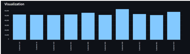
Visualization
