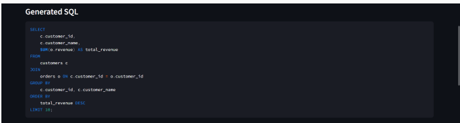
Generated SQL
