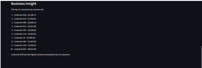
Business insight
