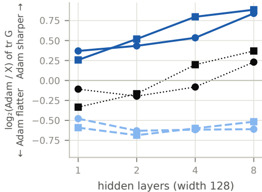
(a) Adam vs SGD
