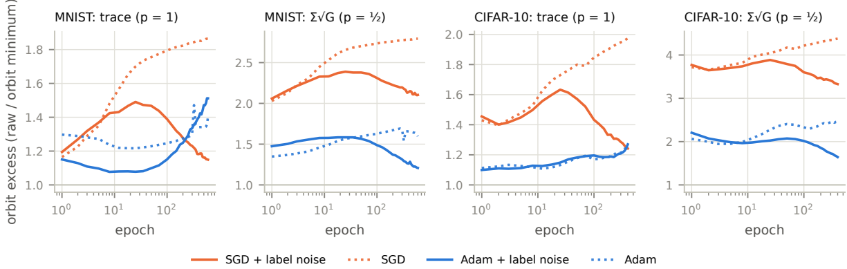
Figure 5: Where each optimizer drifts on long horizons. Orbit excess for the trace ( p = 1 ) and for \sum_i \sqrt{G_{ii}} ( p = \frac{1}{2} ) during 600 (MNIST) and 400 (CIFAR-10) epochs, with and without label noise (SGD \eta = 0.12 , Adam \eta = 6 \times 10^{-4} , batch size 128; mean of two seeds; log-scaled epoch axis). Without label noise SGD’s coordinates freeze once the data are fit. With label noise SGD moves toward the trace-minimizing point, and Adam moves toward the \sum_i \sqrt{G_{ii}} -minimizing point while its trace excess grows: the destinations predicted for label-noise SGD [6, 9] and for Adam [25].
