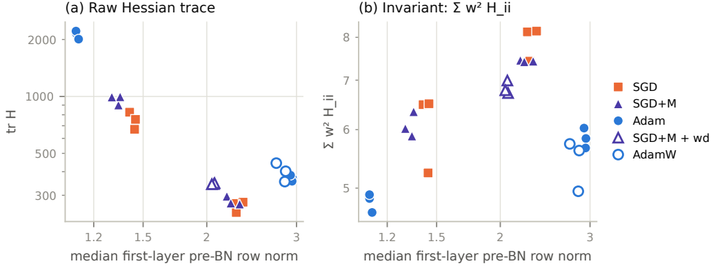
Figure 9: BatchNorm MLP on CIFAR-10 at training loss 0.1 (one point per run). (a) The raw Hessian trace is almost a function of the pre-BN weight norm, which the learning rate sets; Adam at 3 \times 10^{-4} (left) looks sharpest and Adam at 10^{-3} (right) looks about as flat as SGD. (b) \sum_i w_i^2 H_{ii} , invariant to every per-weight rescaling, does not follow the norm. It ranks every Adam run at 3 \times 10^{-4} below all twelve SGD and SGD+M runs without weight decay, and every Adam run at 10^{-3} below at least nine of them. Hollow markers: with weight decay.
