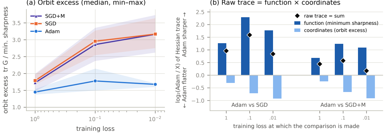
Figure 8: CNN on CIFAR-10. (a) Orbit excess at matched training loss; rescaling acts on convolutional channels, through max-pooling and the flatten into the dense layer. (b) Exact split of the Adam/X trace ratio. On this network Adam’s solutions are sharper at the function level, and the coordinate term, which again favours Adam and grows during training, hides most of that difference.
