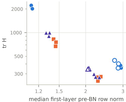
(a) Raw Hessian trace
