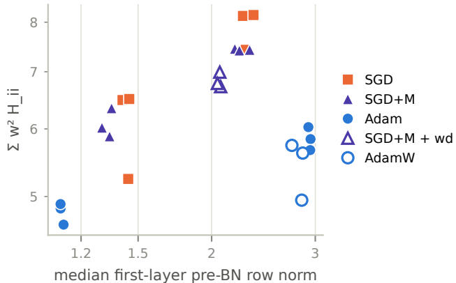
(b) Invariant: \sum w^2 H_{ii}
