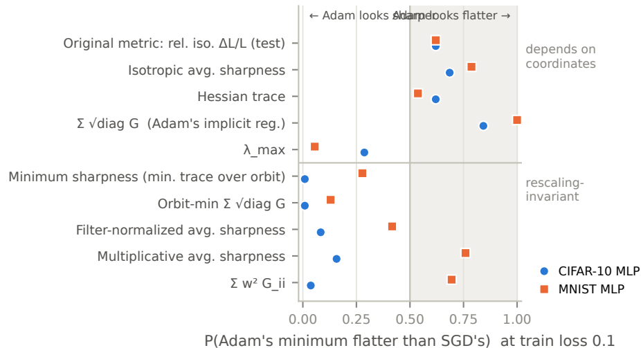
(a) The optimizer ordering flips with the measure
