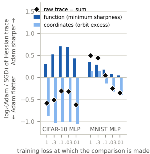
(b) Raw trace = function \times coordinates (exact)
