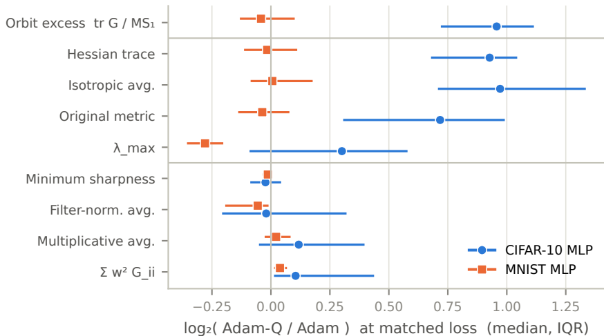
Removing Adam's symmetry drift: raw sharpness rises, invariant sharpness does not
