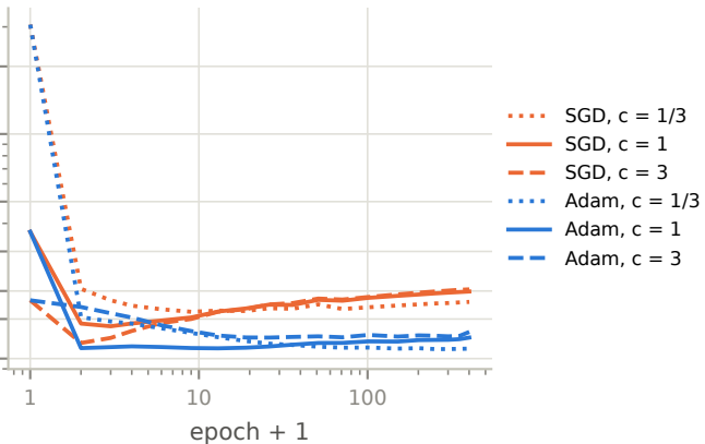
(b) CIFAR-10 MLP, no label noise
