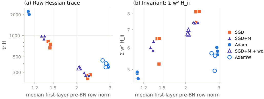
Figure 10: BatchNorm MLP on CIFAR-10 at training loss 0.1 (one point per run). (a) The raw Hessian trace is almost a function of the pre-BN weight norm, which the learning rate sets; Adam at 3 \times 10^{-4} (left) looks sharpest and Adam at 10^{-3} (right) looks about as flat as SGD. (b) \sum_i w_i^2 H_{ii} , invariant to every per-weight rescaling, does not follow the norm. It ranks every Adam run at 3 \times 10^{-4} below all twelve SGD and SGD+M runs without weight decay, and every Adam run at 10^{-3} below at least nine of them. Hollow markers: with weight decay.
