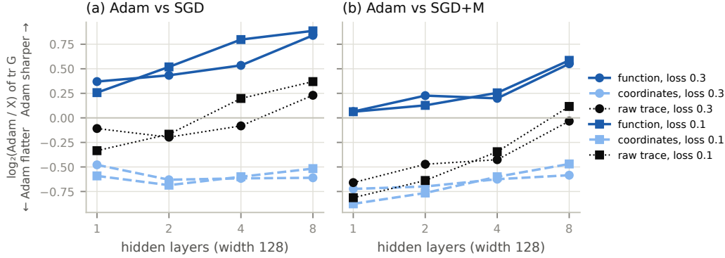
Figure 9: Depth. Exact split (2) of the Adam/X trace ratio for CIFAR-10 MLPs with 1–8 hidden layers of width 128 (three seeds each). The coordinate term is about the same at every depth; the function term grows with depth, so the coordinate factor reverses the raw ordering in shallow networks and masks the difference in deep ones.
