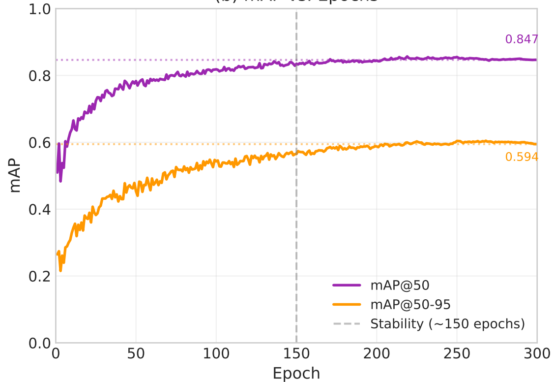
(b) mAP vs. Epochs
