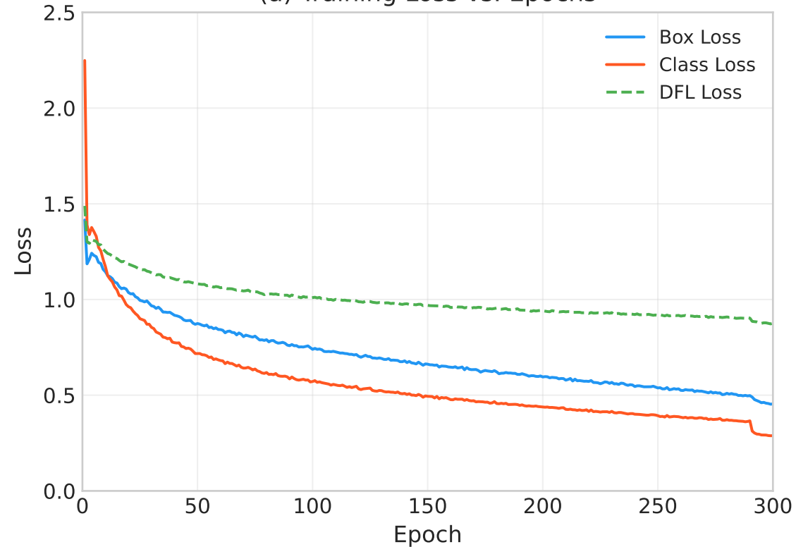
(a) Training Loss vs. Epochs
