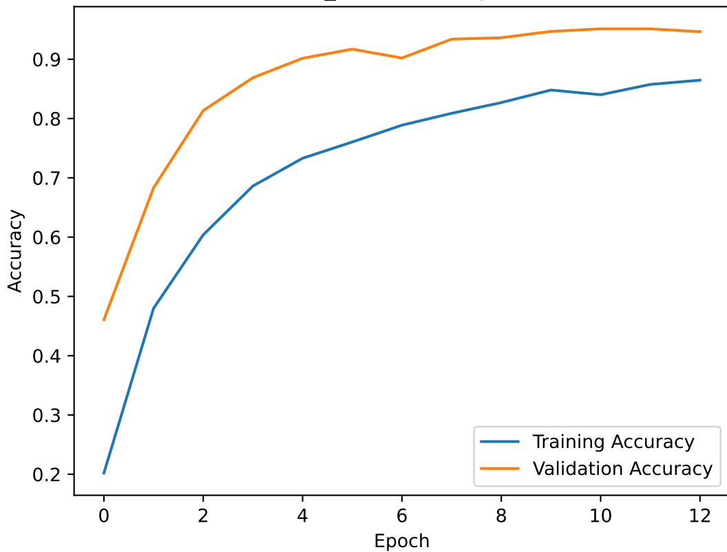
Custom_CNN Accuracy Curve
