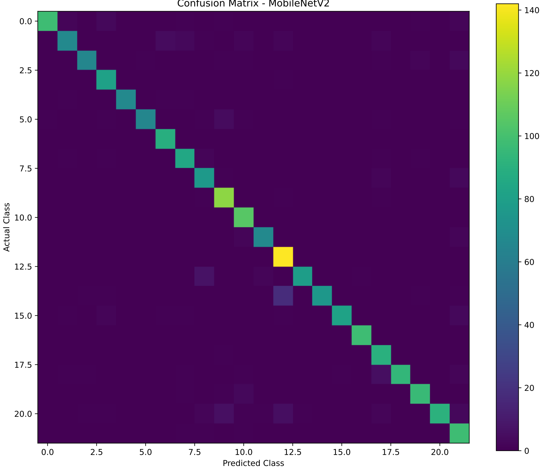
Confusion Matrix - MobileNetV2
