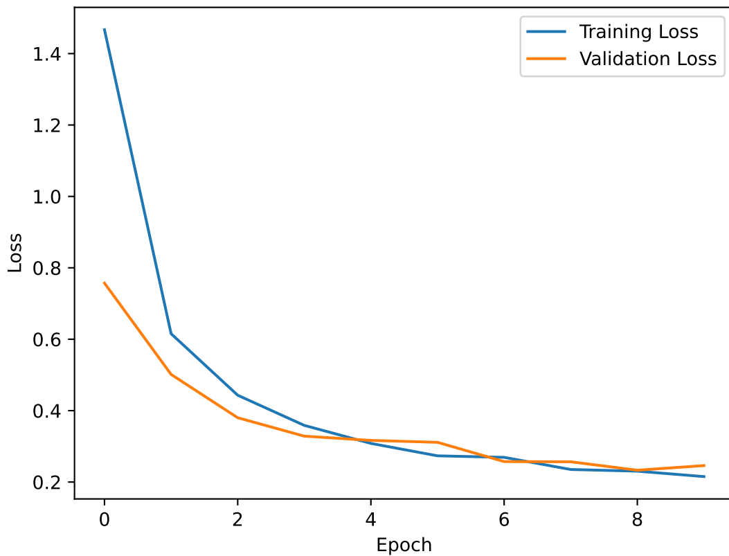
MobileNetV2 Loss Curve
