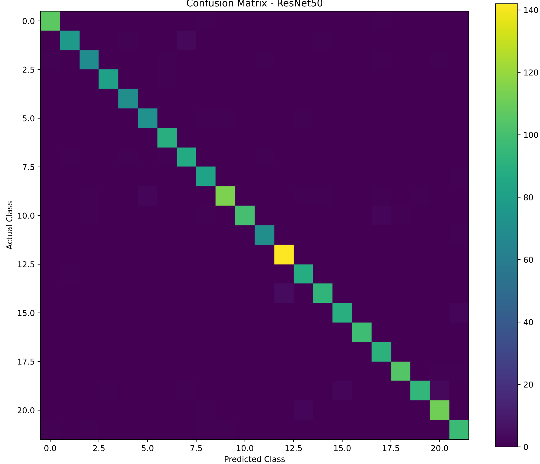
Confusion Matrix - ResNet50
