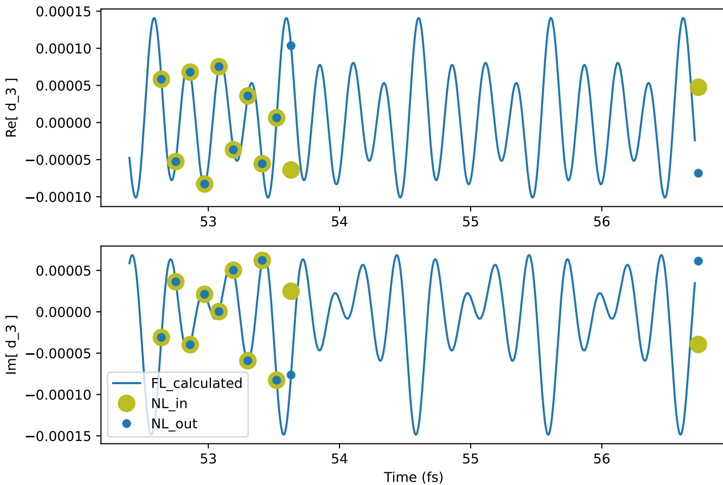
Time-dependent projection over Kohn-Sham state: 3
