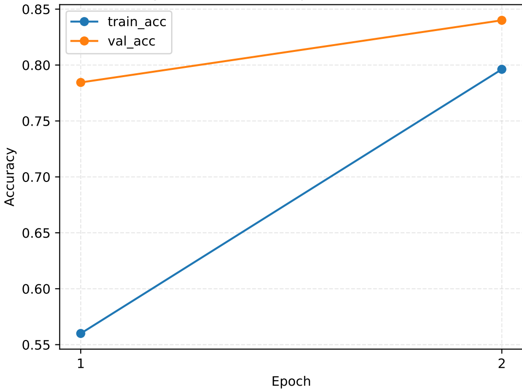
RQ1: Training curve (ResNet18 pretrained, frozen backbone)
