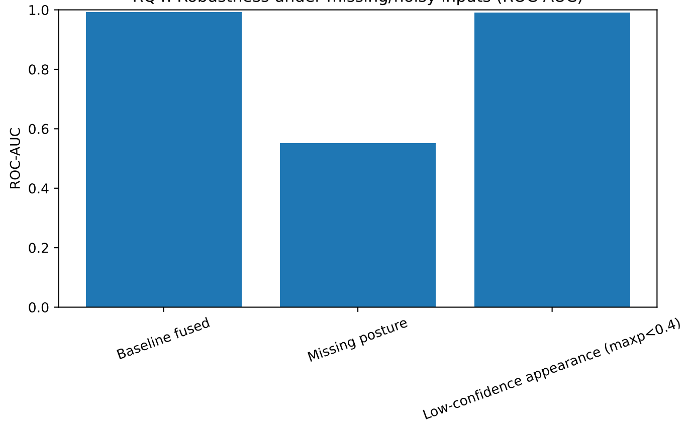
RQ4: Robustness under missing/noisy inputs (ROC-AUC)
