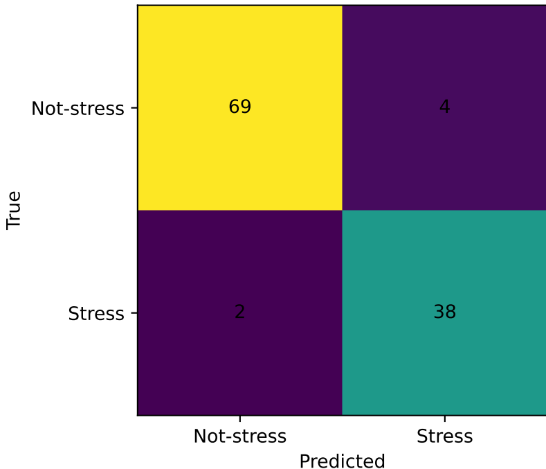
RQ3: Confusion matrix (Fused model)
