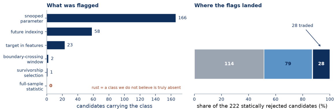
Figure 2. Left: what the static auditor found across all 1,550 sources, by class. One class dominates and one is empty, and the empty one is the finding; see below. Right: what became of the 222 candidates it rejected. Almost every flag landed on code that never took a position , so a leakage-prevalence rate measured over generated source is not a deployment-risk rate.
