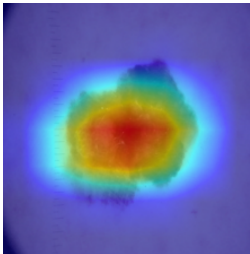
Grad-CAM Heatmap
