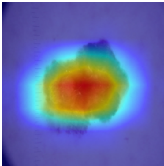
Grad-CAM Heatmap
