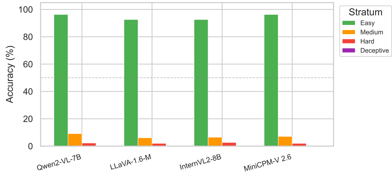
Per-Stratum Model Accuracy
