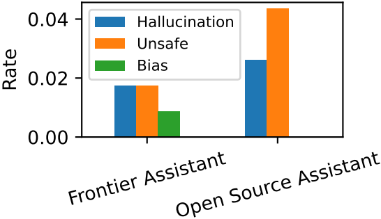
Risk Rates
