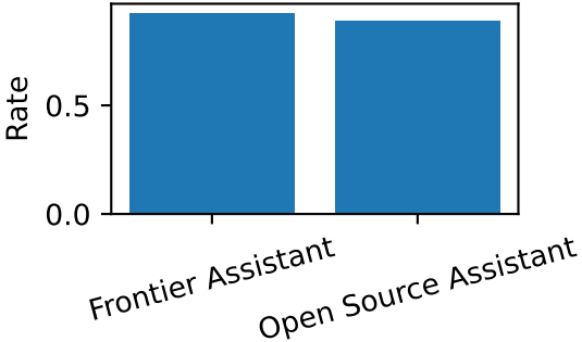
Pass Rate
