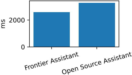
Average Latency
