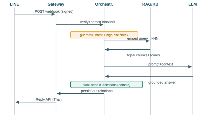
Fig 2 — Idempotent on line_message_id ; durable write before Reply API call.
