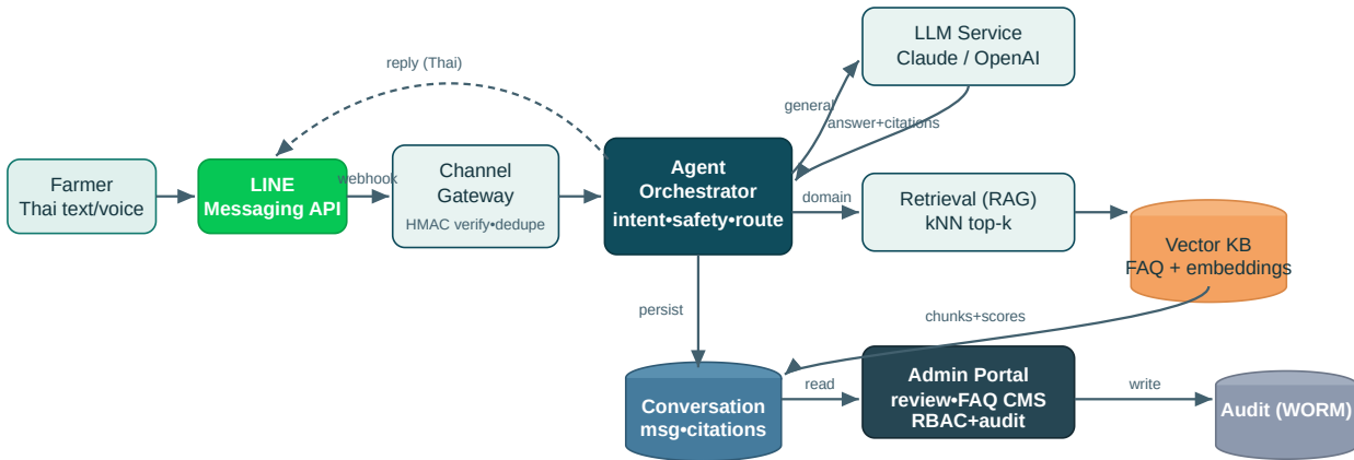
Fig 1 — C4 container view. Stateless gateway/orchestrator; strong-consistency stores for conversation & knowledge; append-only audit.
