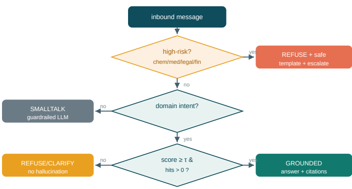
Fig 3 — Policy enforced in orchestrator, independent of model output ( \tau = RETRIEVAL_MIN_SCORE).
