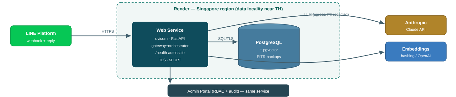
Fig 5 — Blueprint-provisioned (render.yaml). Secrets (LINE, Anthropic) injected as env; ADMIN_TOKEN auto-generated; DATABASE_URL bound from managed DB.
