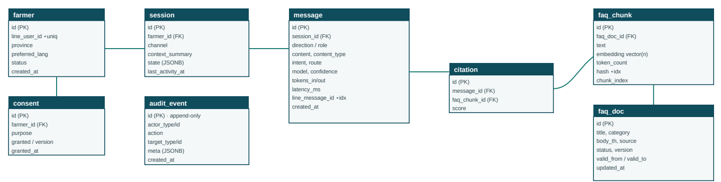
Fig 4 — UUID PKs (string-portable SQLite → Postgres). faq_chunk.embedding = JSON array on SQLite / native pgvector in prod. Erasure cascades farmer → session → message → citation + media/embeddings; audit retained lawfully.
