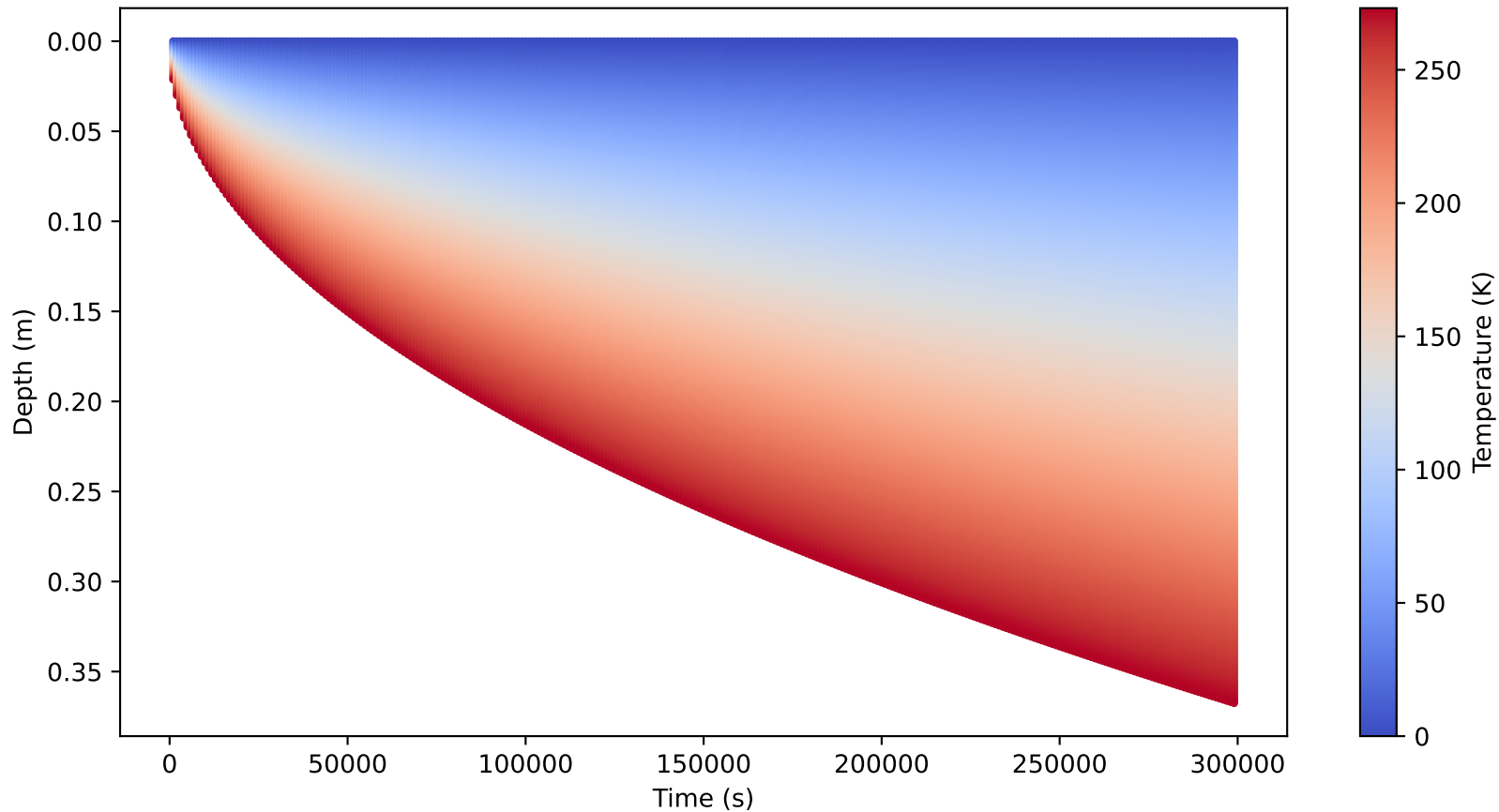
Temperature evolution Analytical
