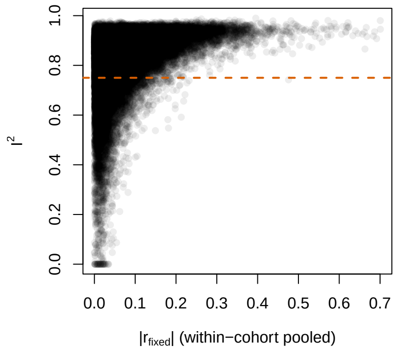
B I^2 vs effect size
