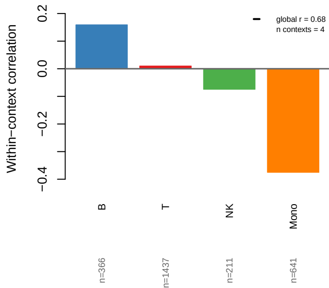
B Context correlations
