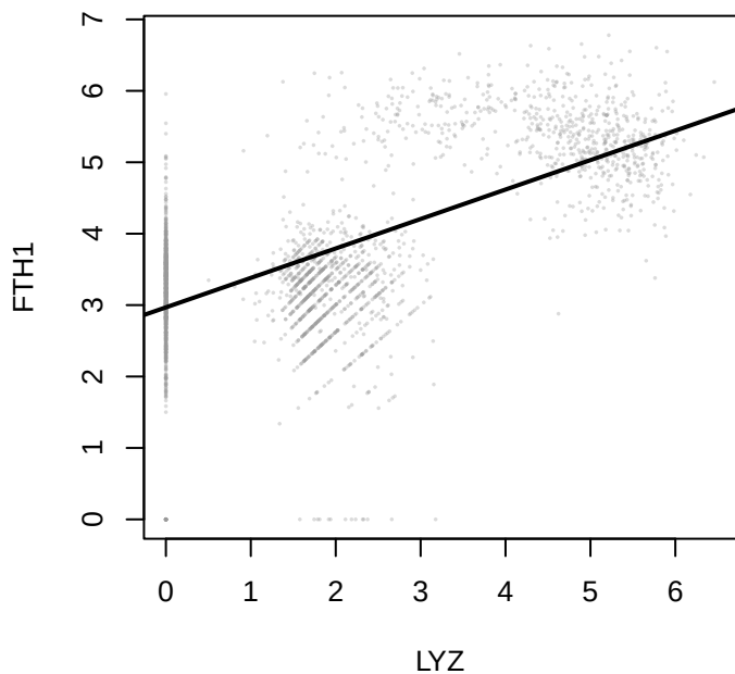
A Global r = 0.677
