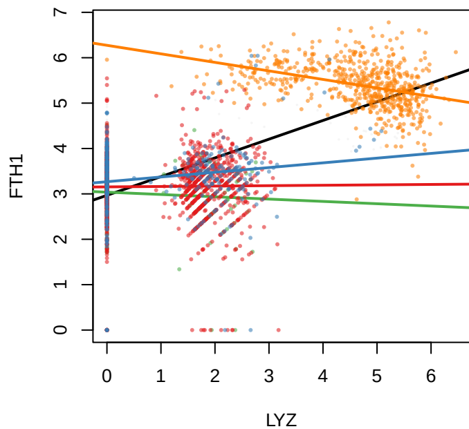
D Filtered contexts (resid r = -0.038 )
