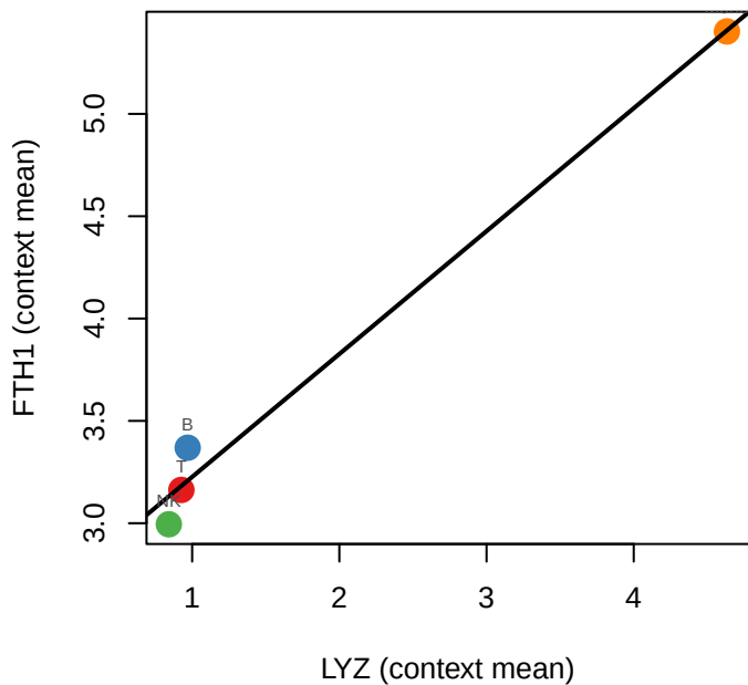
C Context means r = 0.994
