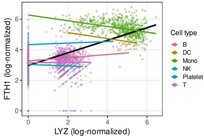
PBMC: LYZ vs FTH1 (global r = +0.68 )
