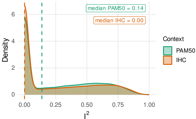
Distribution of I^2 by context
