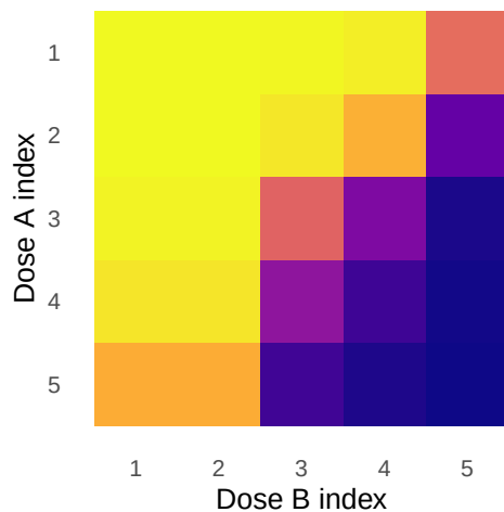
\hat{\theta}_{\text{add}} (viability)
