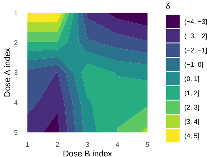
Interaction contour
