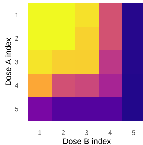
\hat{\theta}_{\text{iso}} (viability)
