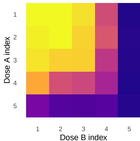
Observed viability
