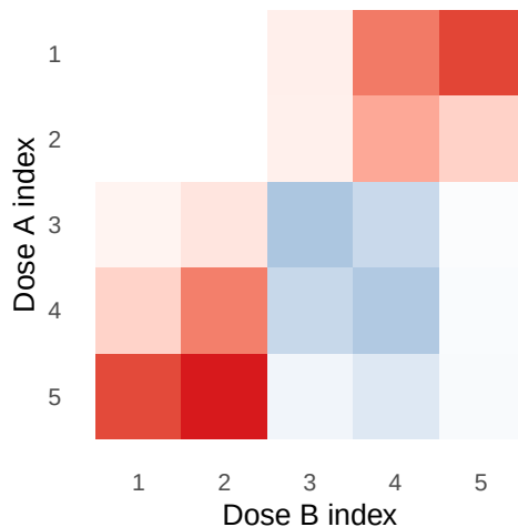
S_{\text{SIR}} (viability)
