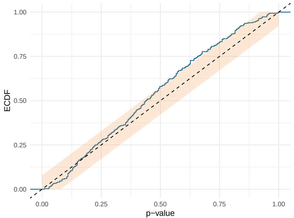
Pseudo-null p-value distribution
