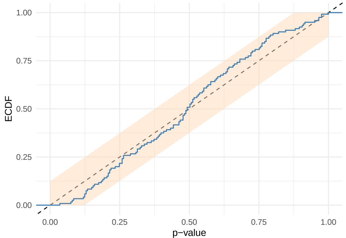
Pseudo-null p-value distribution
