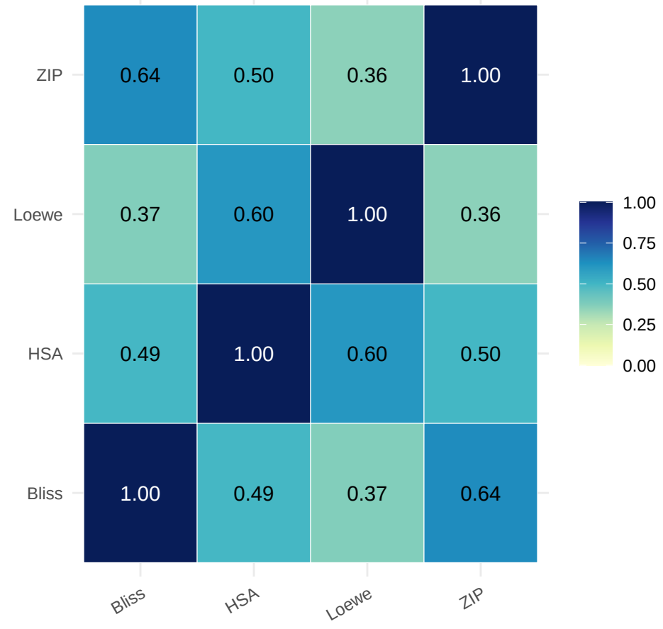
Jaccard overlap of top-5% hits
