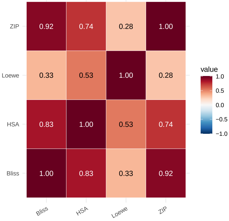
Pearson correlation of synergy scores
