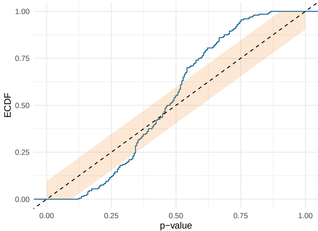
Null p-value distribution
