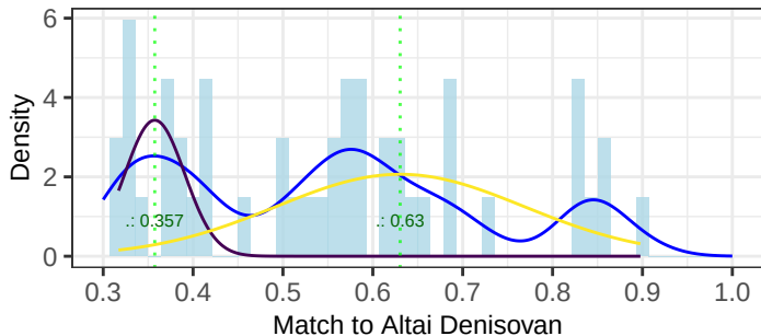
C152-CKZ06-Mat : GMM Fit with 3 Components
