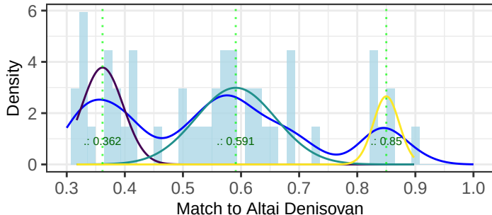
C152-CKZ06-Mat : GMM Fit with 3 Components
