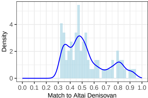
HG02106_hap2 : GMM Fit with 1 Components
