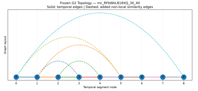
Fig. 1. Supplied G2 example for track mc_RfBwKl818XQ_30_40 . Temporal and sparse nonlocal links connect mean-pooled audio segments.
