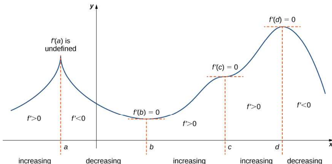
Figure 4.31 The function f has four critical points: a , b , c , and d . The function f has local maxima at a and d , and a local
