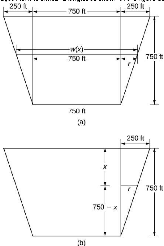
Figure 6.61 We use similar triangles to determine a function for the width of the dam. (a) Assumed dimensions of the dam; (b) highlighting the similar triangles.
