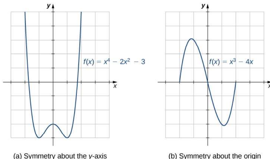
Figure 1.13 (a) A graph that is symmetric about the y -axis. (b) A graph that is symmetric about the origin.
