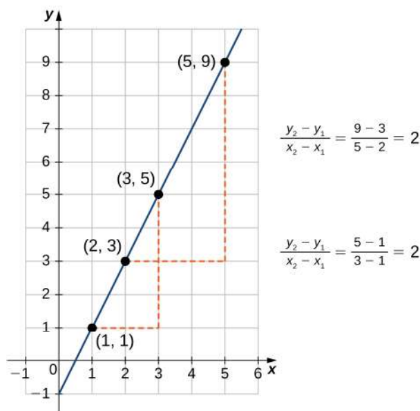
Figure 1.16 For any linear function, the slope (y_2 - y_1)/(x_2 - x_1) is independent of the choice of points (x_1, y_1) and (x_2, y_2) on the line.
